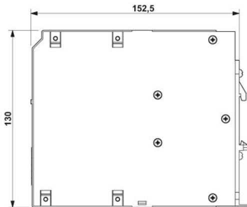
Dimensioned drawing
