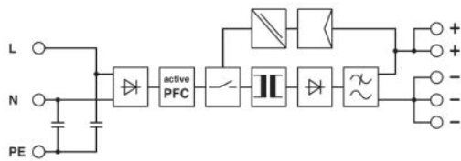
Block diagram
